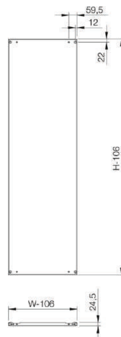
Mounting plate
