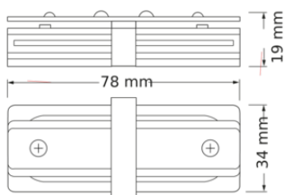
TRACK 1-PH CONNECTOR I TYPE
