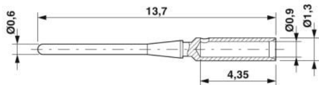
Dimensional drawing
