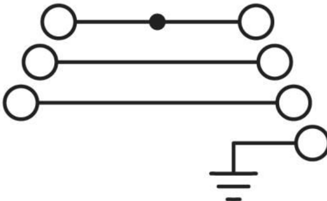
Circuit diagram
