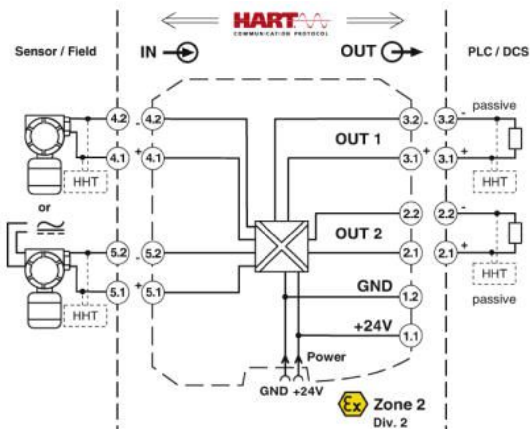
Block diagram
