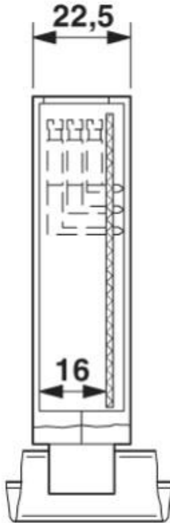
Dimensional drawing
