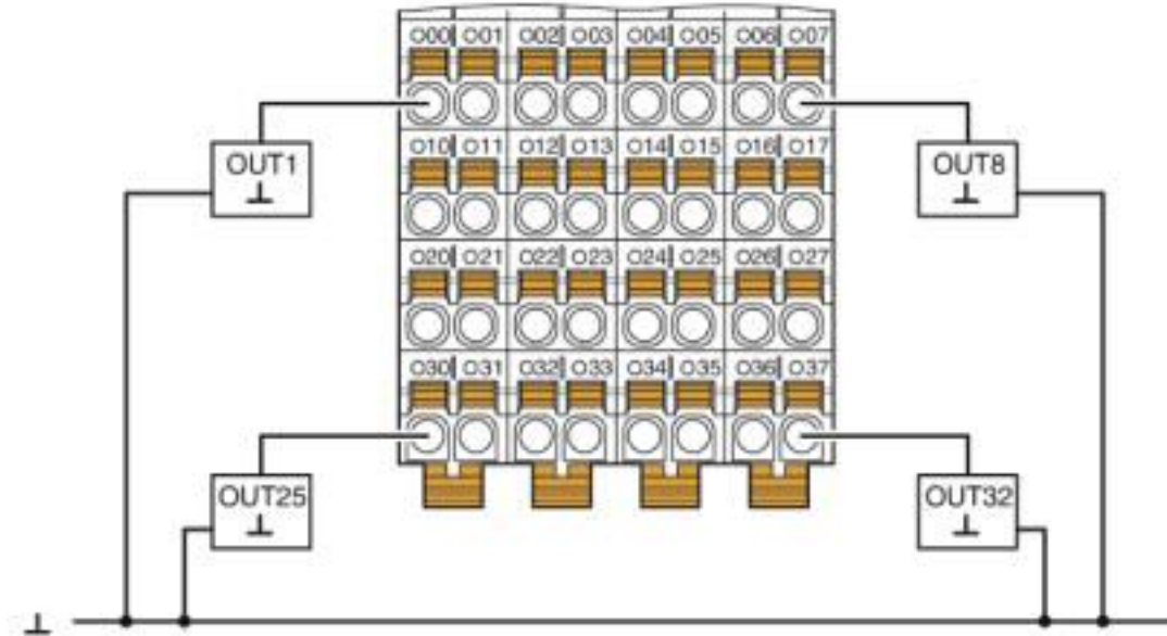
Connection diagram
