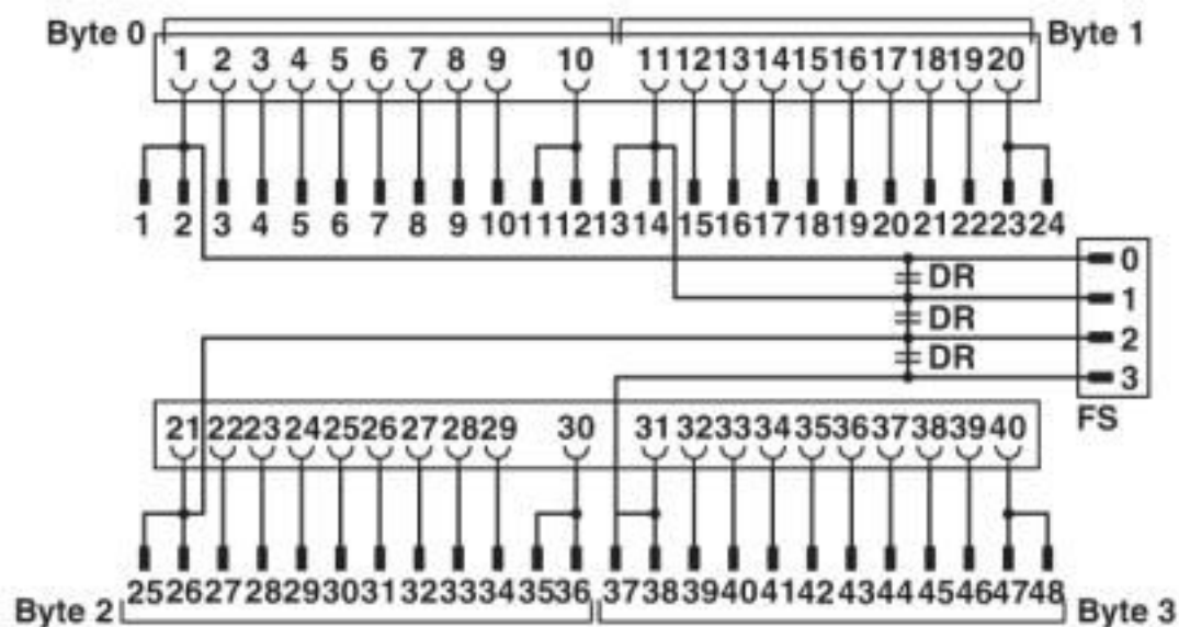
Connection scheme FLKM 50-PA-S300
