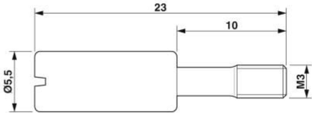
Dimensional drawing
