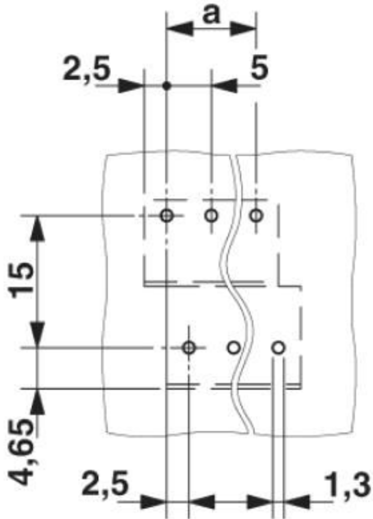
Drilling diagram
