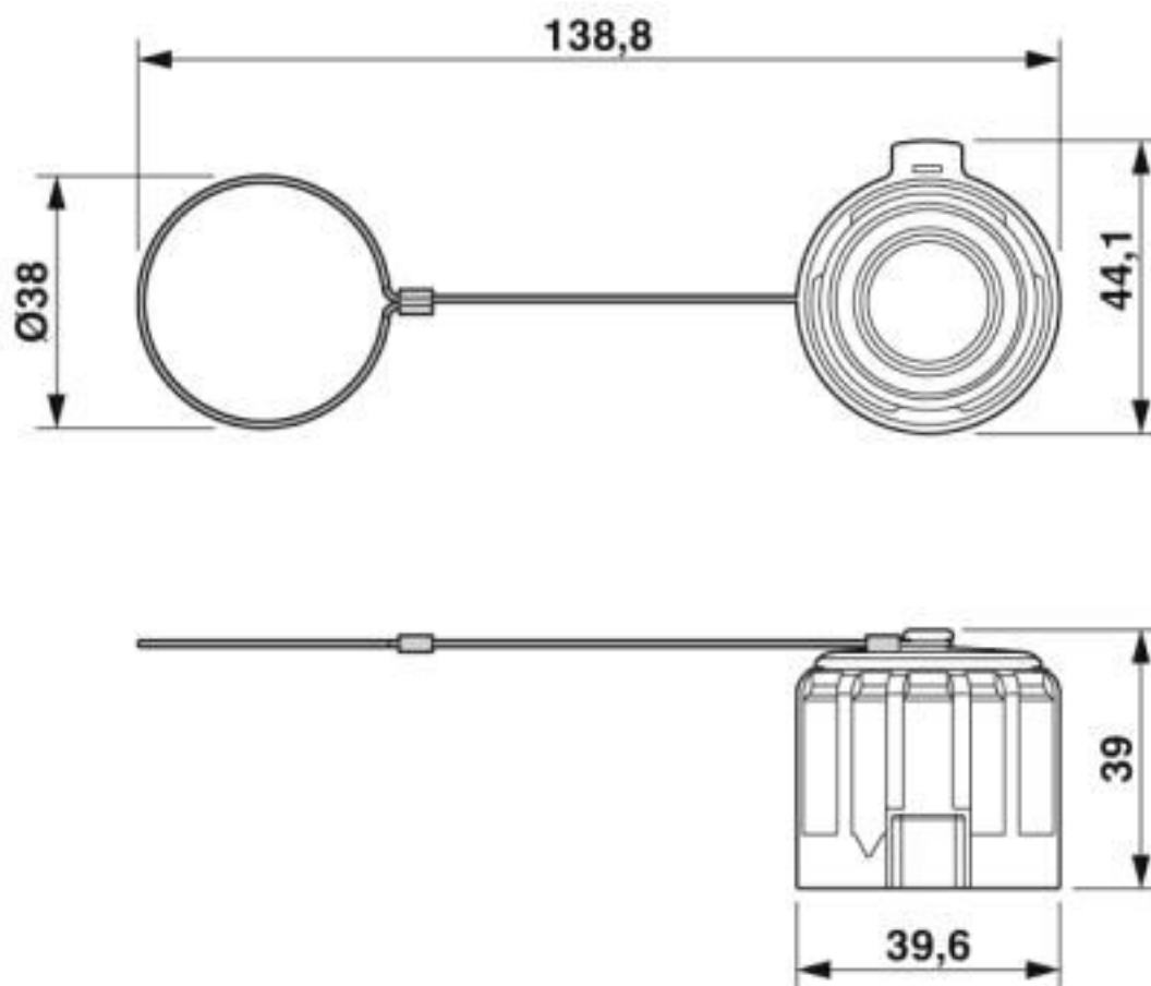
Dimensional drawing
