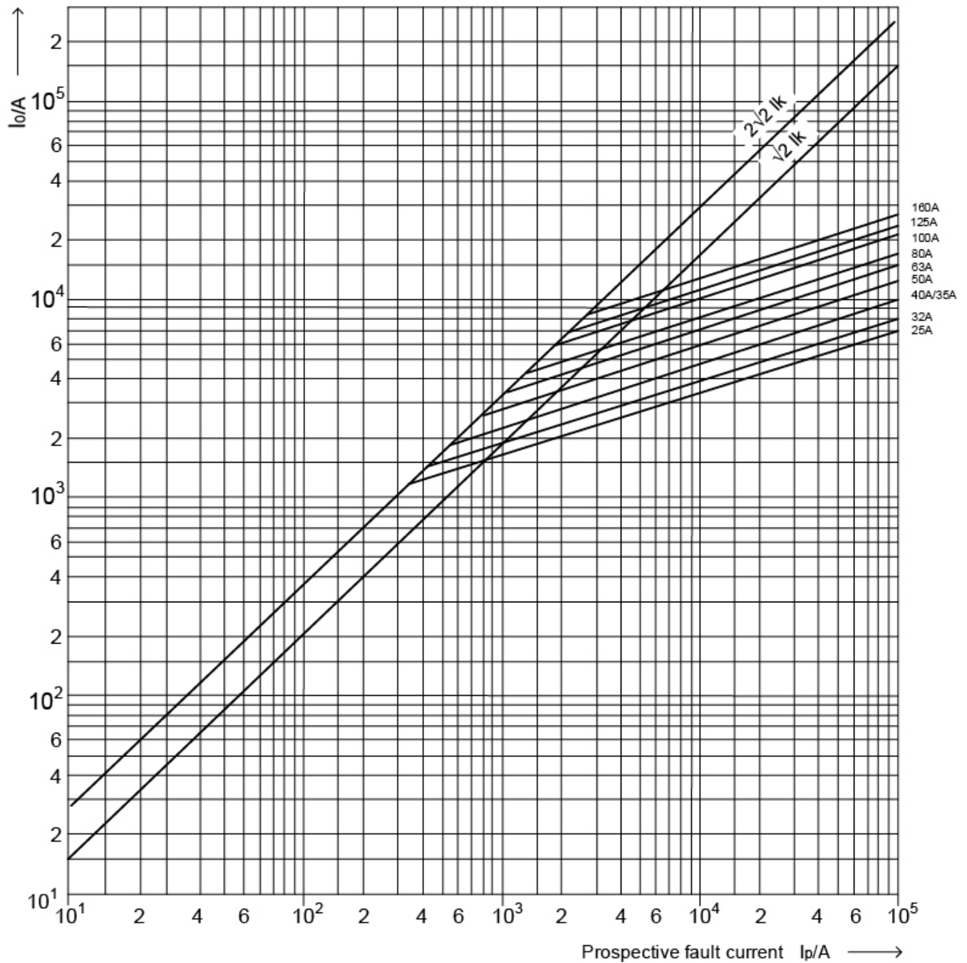
Cut-off characteristics
