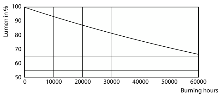
Lumen Maintenance Diagram - TrueForce LED HPL ND 60-42W E40 840
