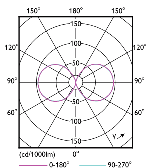
Light Distribution Diagram - TrueForce LED HPL ND 60-42W E40 840
