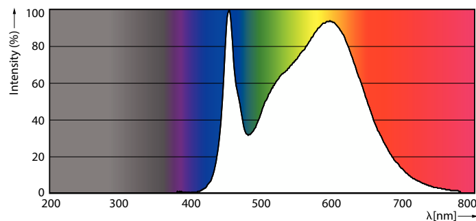
Spectral Power Distribution Colour - TrueForce LED HPL ND 60-42W E40 840
