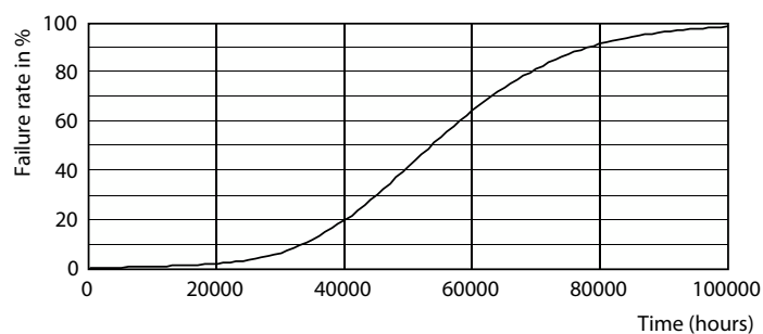
Life Expectancy Diagram - TrueForce LED HPL ND 60-42W E40 840
