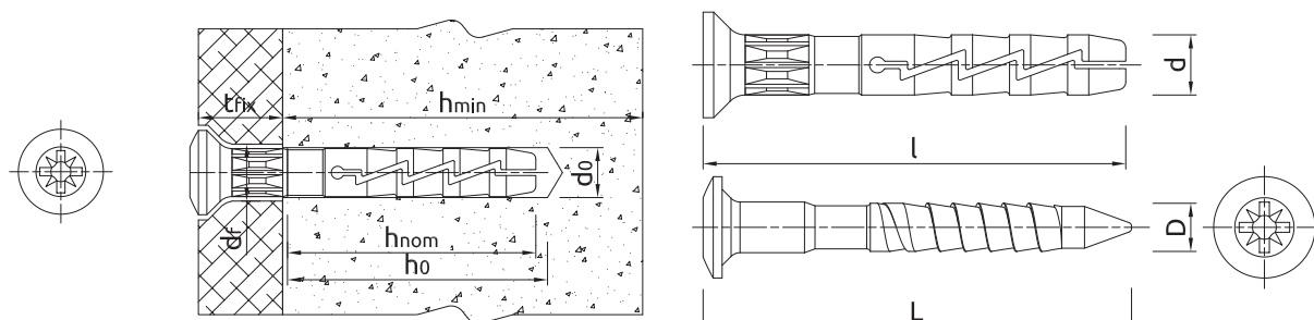
Installation data
